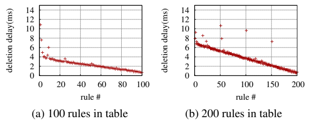
Figure 9: Vendor B per-rule del. latency: same priority
