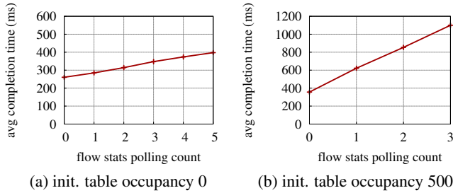
Figure 12: Polling effects on completion time on Vendor A switch. Burst size 100. Measured using simple openflow rules (i.e., just vary destination IP).
