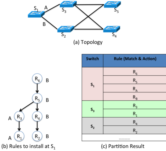
Figure 17: Illustration of rule offloading
