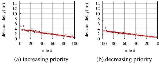
Figure 11: Vendor B priority per-rule deletion latency results, burst size 100: (a) increasing priority (b) decreasing priority
