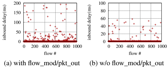
Figure 3: Inbound delay on Vendor B. Flow arrival rate = 200/s
