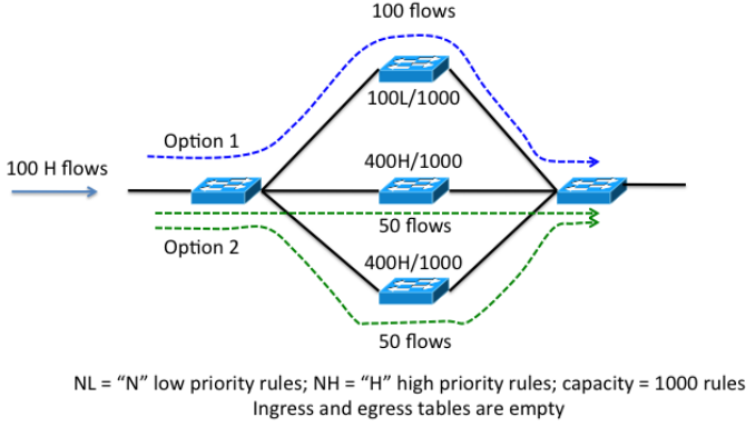
Figure 16: Illustration of flow engineering assuming a Vendor A switch
