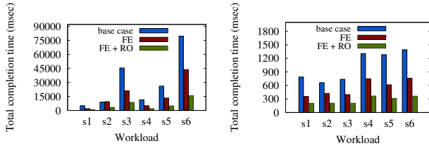
(a) Latency on Vendor A switch (b) Latency on Vendor B switch
