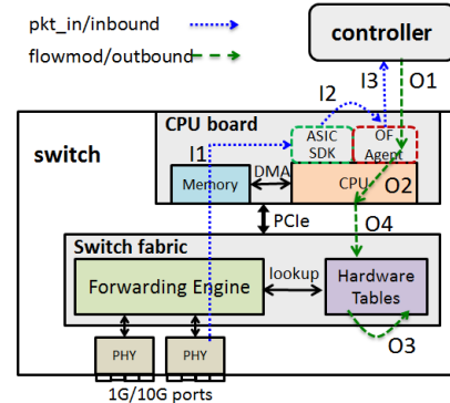
Figure 1: Schematic of an OpenFlow switch. Different rectangular blocks indicate different components of a switch; different boxes do not mean different chips. We also show the factors contributing to inbound and outbound latency
