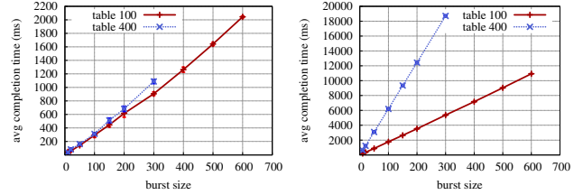
Figure 13: Overall completion time on Vendor A switch. Two priority effects. Initial flow table occupancy is S high (low) priority rules. Then, insert a burst of low (high) priority rules. Averaged on 5 rounds.
