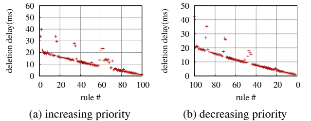
Figure 10: Vendor A priority per-rule deletion latency results, burst size 100: (a) incr. priority (b) decr. priority
