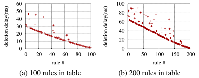
Figure 8: Vendor A per-rule del. latency: same priority
