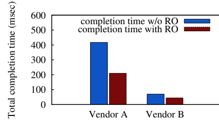
Figure 20: Flow setup time of MicroTE with and without RO in a Fat Tree (k=8) topology
