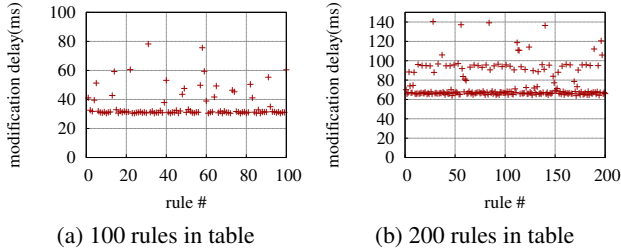
Figure 6: Vendor A per-rule mod. latency: same priority
