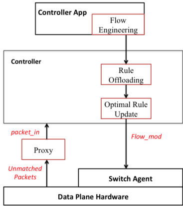
Figure 15: Mazu framework
