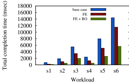
Figure 19: Worst case flow setup time of affected flows in failover scenario with base case, FE and FE+RO techniques in a full mesh (25 nodes) topology with Vendor A switches
