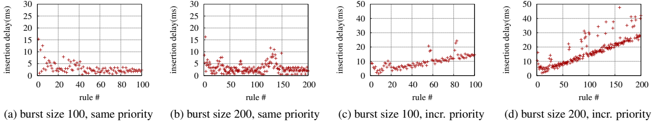
Figure 4: Vendor A priority per-rule insert latency results
